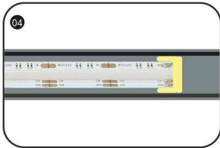
◎ Stick Mylar tape to isolate the cutting position from the bottom of profile inner slot to avoid short-circuit;
