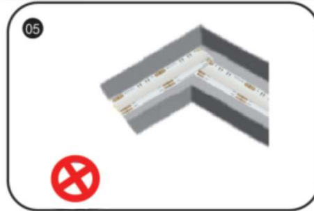
◎ The installation at the corner is shown as the above figure. △ Notes: No bending it into right angle; No twisting it to stick on the mounting surface.
